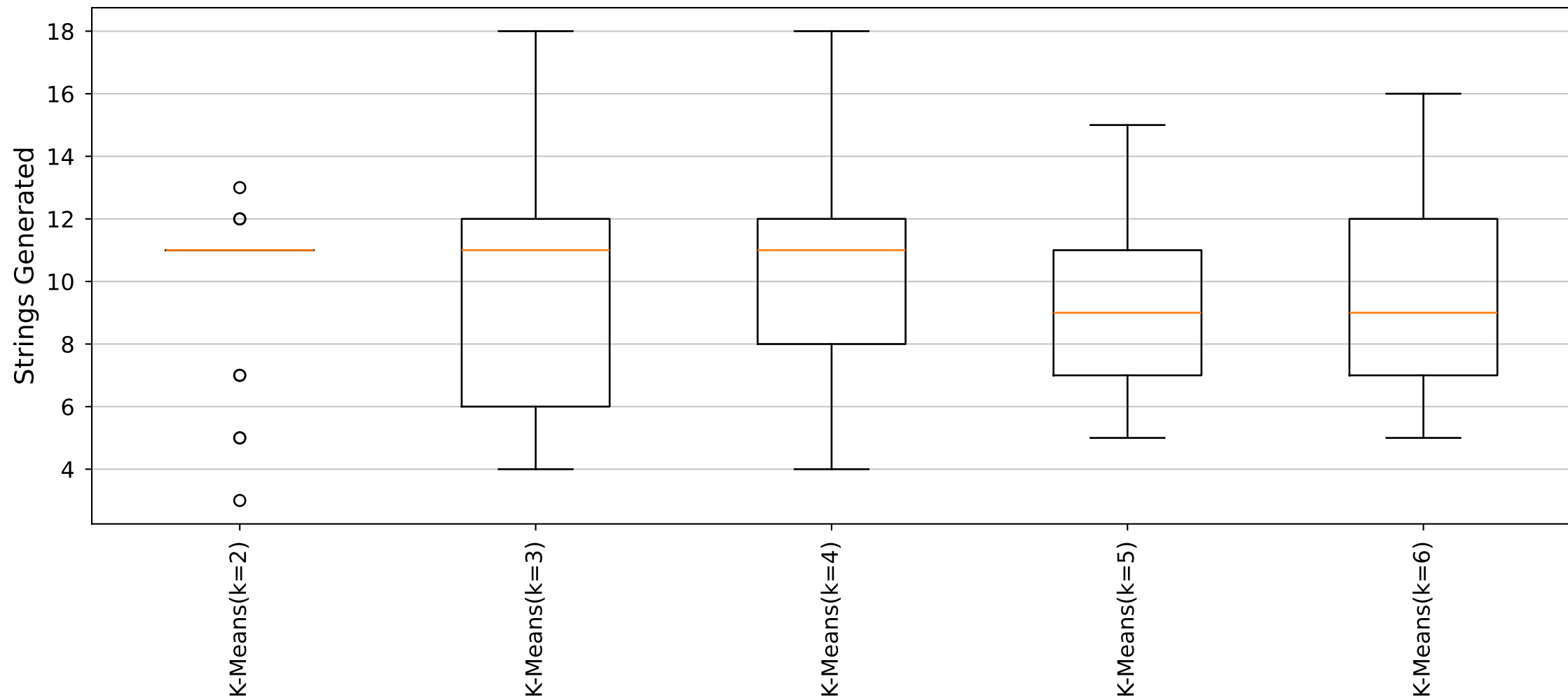
YARA Rules Strings Generated Distribution (Cluster21_Size6 dataset)
